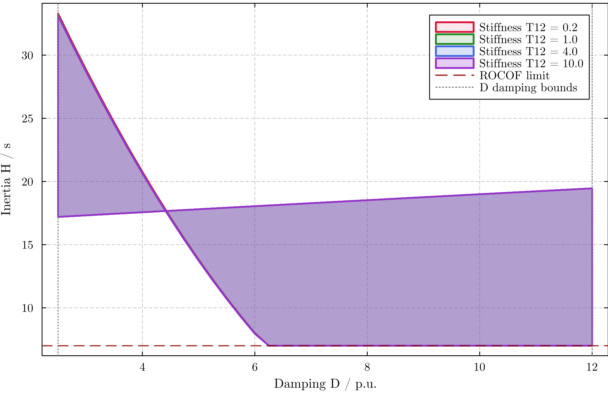
Impact of Tie-line Stiffness T12 on Area 1 Security Region
